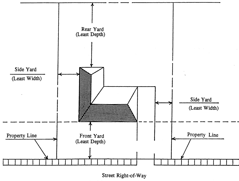
Figure 4: Yard Definitions
